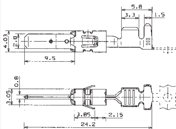
Male terminals
