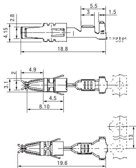
Female terminals
