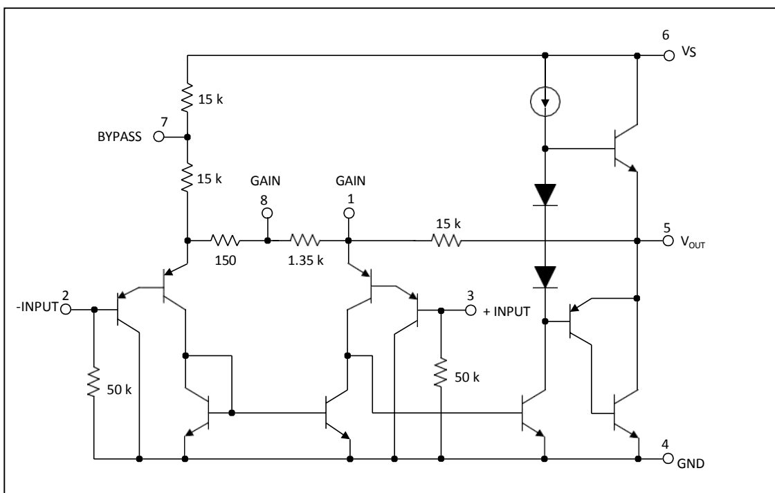
schematic diagram
