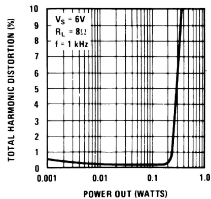
Figure 6-6. Total Harmonic Distortion vs Power Out
