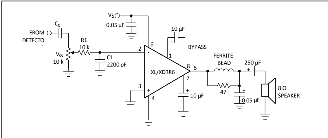
Figure 8-13. AM Radio Power Amplifier
