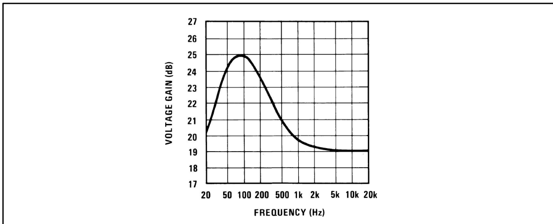
Figure 8-10. Voltage Gain vs Frequency
