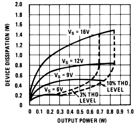
Figure 6-8. Device Dissipation vs Output Power
