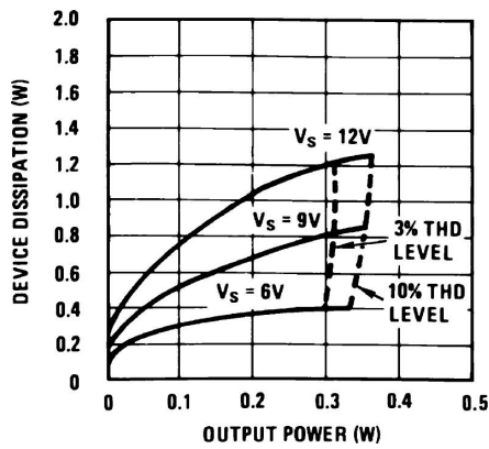
Figure 6-7. Device Dissipation vs Output Power
