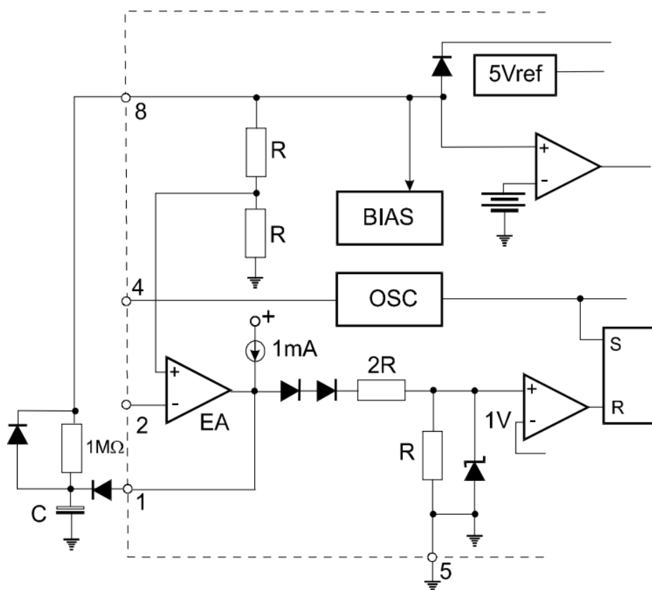
Figure 8. Soft-Start Circuit
