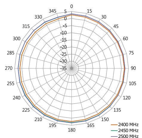
XY-Plane Gain
