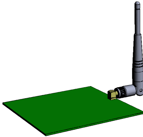
Figure 11. On edge of ground plane, Bent 90 Degrees
