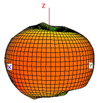
2500 MHz
