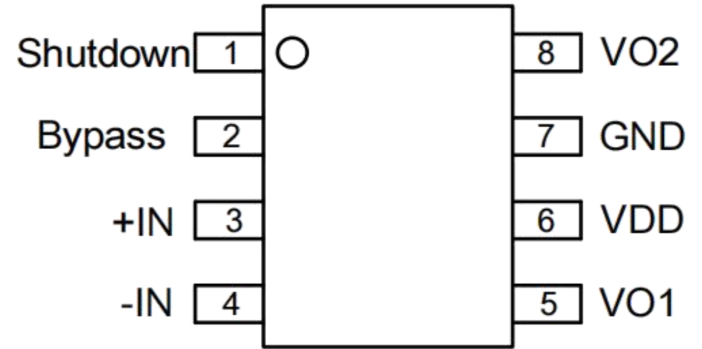
TPA311 Pin Diagram
