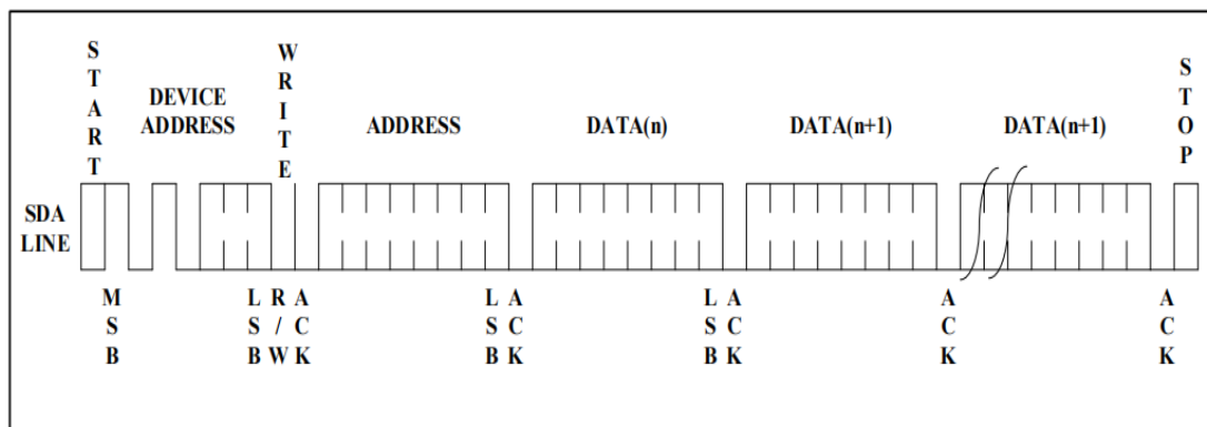
Figure 8. Page Write
