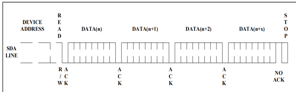
Figure 11. Sequential Read
