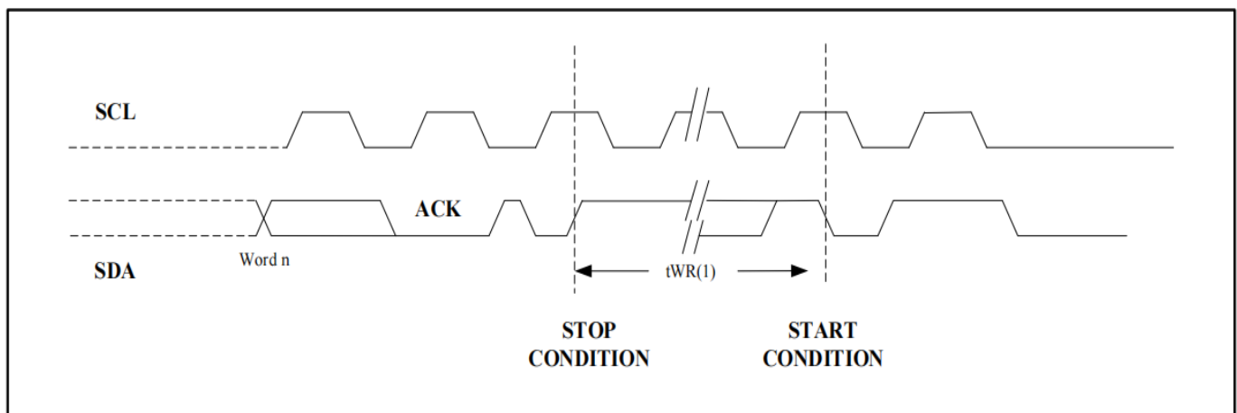
Figure 13. SCL: Serial Clock, SDA: Serial Data I/O
