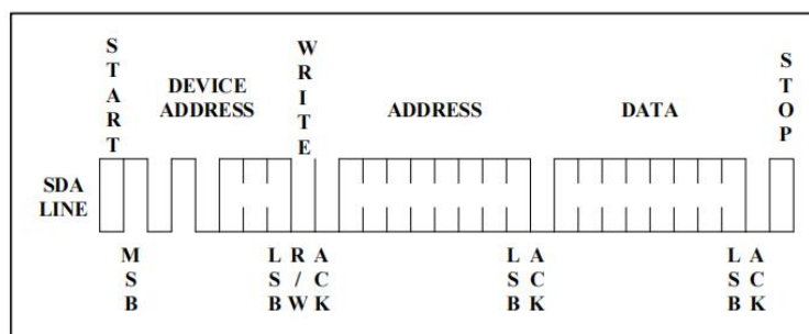
Figure 7. Byte Write
