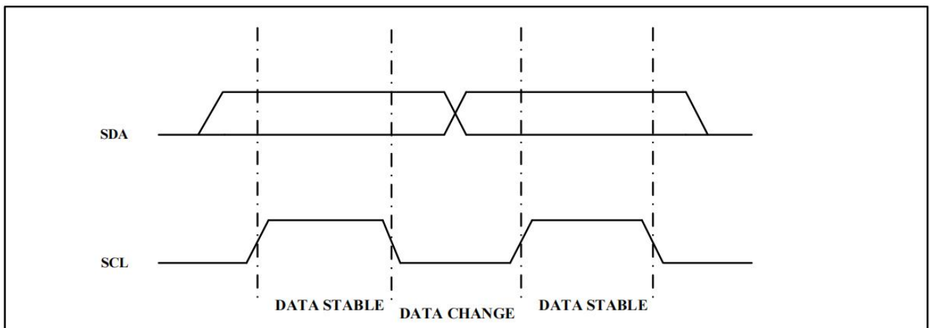
Figure 2. Data Validity
