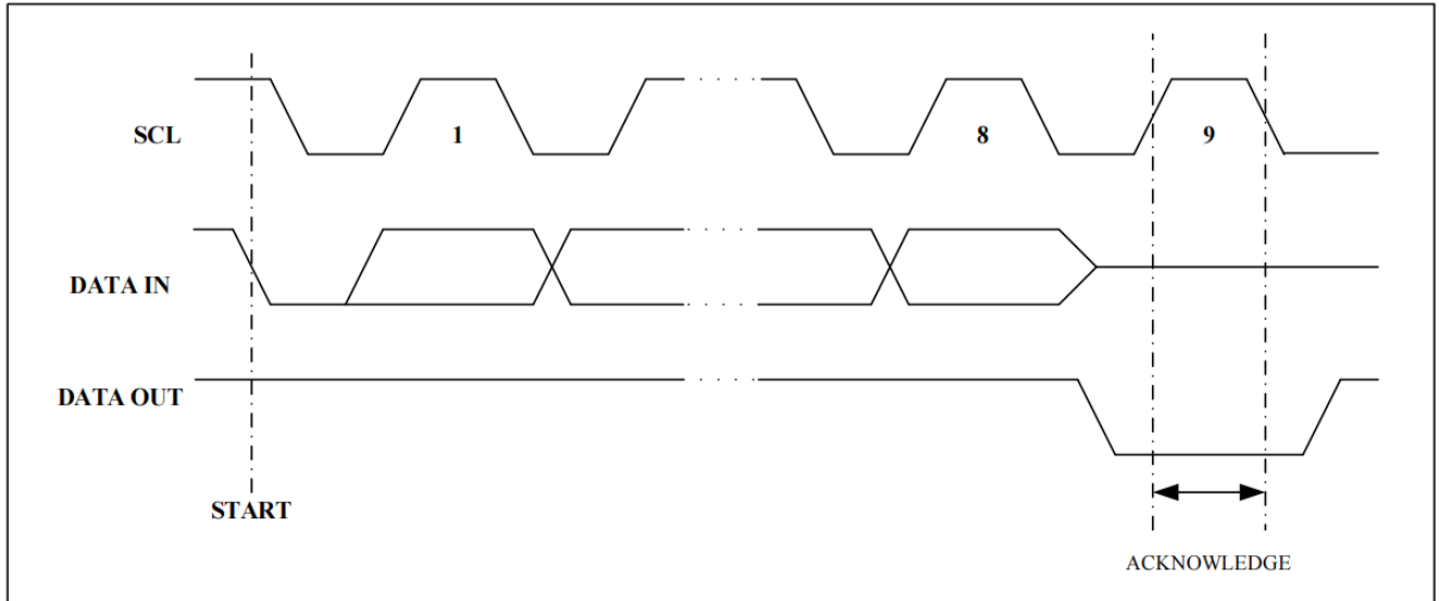
Figure 4. Output Acknowledge
