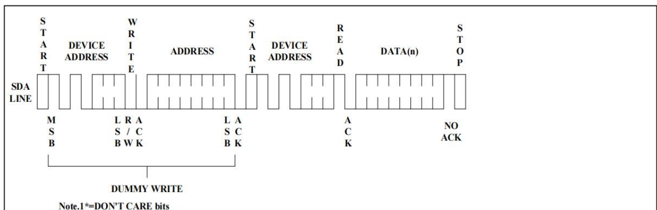
Figure 10. Random Read
