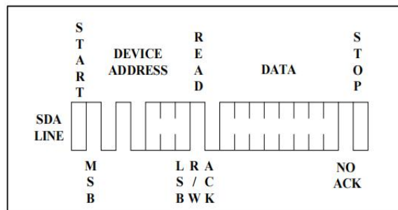
Figure 9. Current Address Read
