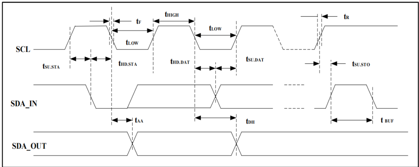
Figure 12. SCL: Serial Clock, SDA: Serial Data I/O
