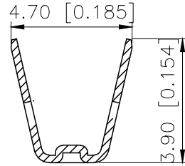
SECTION:A-A SCALE:1:1
