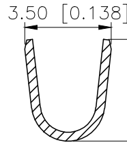
SECTION:B-B SCALE:1:1
