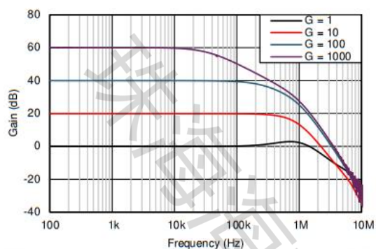
图 1. Gain vs Frequency
