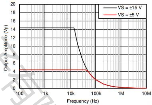
图 16. Maximum Output Voltage vs Frequency
