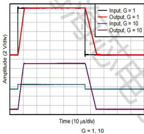
图 21. Large Signal
