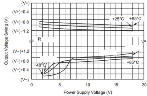
图 14. Output Voltage Swing vs Power Supply Voltage
