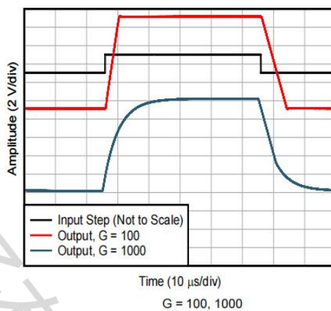
图 22. Large Signal
