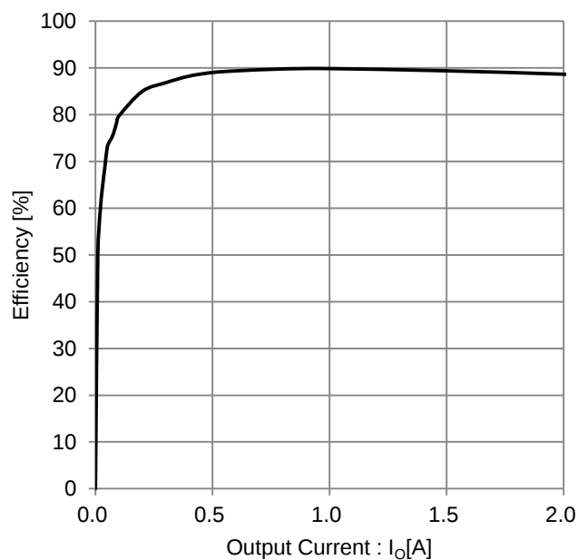
Figure 14. Efficiency vs Output Current (Conversion Efficiency 1 V_{IN} = 13.2 \text{ V} )
