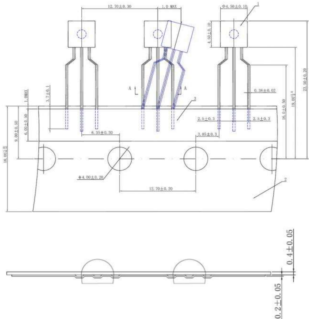
TO-92 (Taping)
