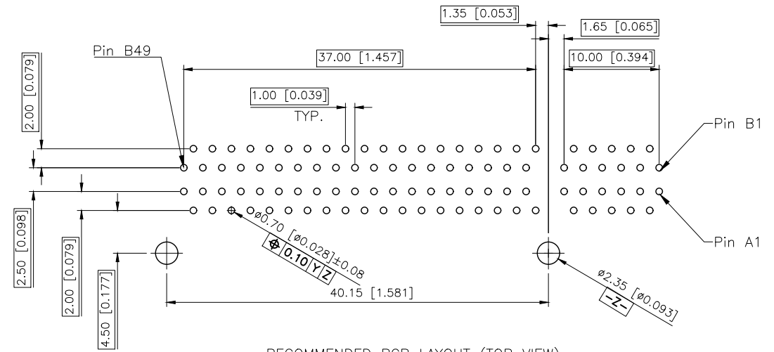
RECOMMENDED PCB LAYOUT (TOP VIEW) FOR 98P TOLERANCE: ±0.05 DATUM Y IS THE PCB SOLDER SURFACE
