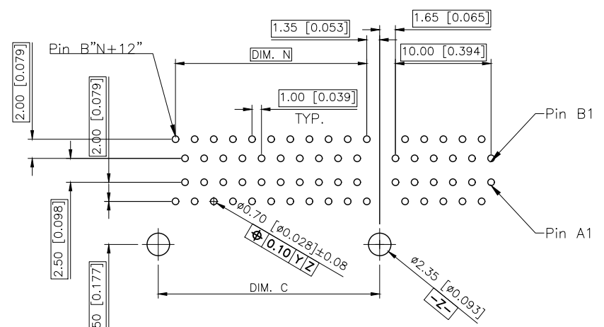
RECOMMENDED PCB LAYOUT (TOP VIEW) FOR 36P, 64P, 164P TOLERANCE: ±0.05 DATUM Y IS THE PCB SOLDER SURFACE
