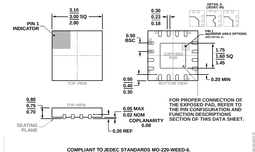
COMPLIANT TO JEDEC STANDARDS MO-220-WEED-6. Figure 41. 16-Lead Lead Frame Chip Scale Package [LFCSP] 3 mm × 3 mm Body and 0.75 mm Package Height (CP-16-22) Dimensions shown in millimeters
