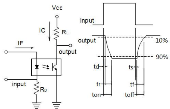
响应时间测试电路 Test Circuit for Response Time
