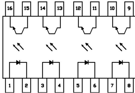
Pin Configuration
