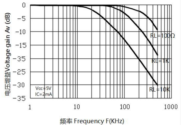
频率响应特性曲线 Frequency Response
