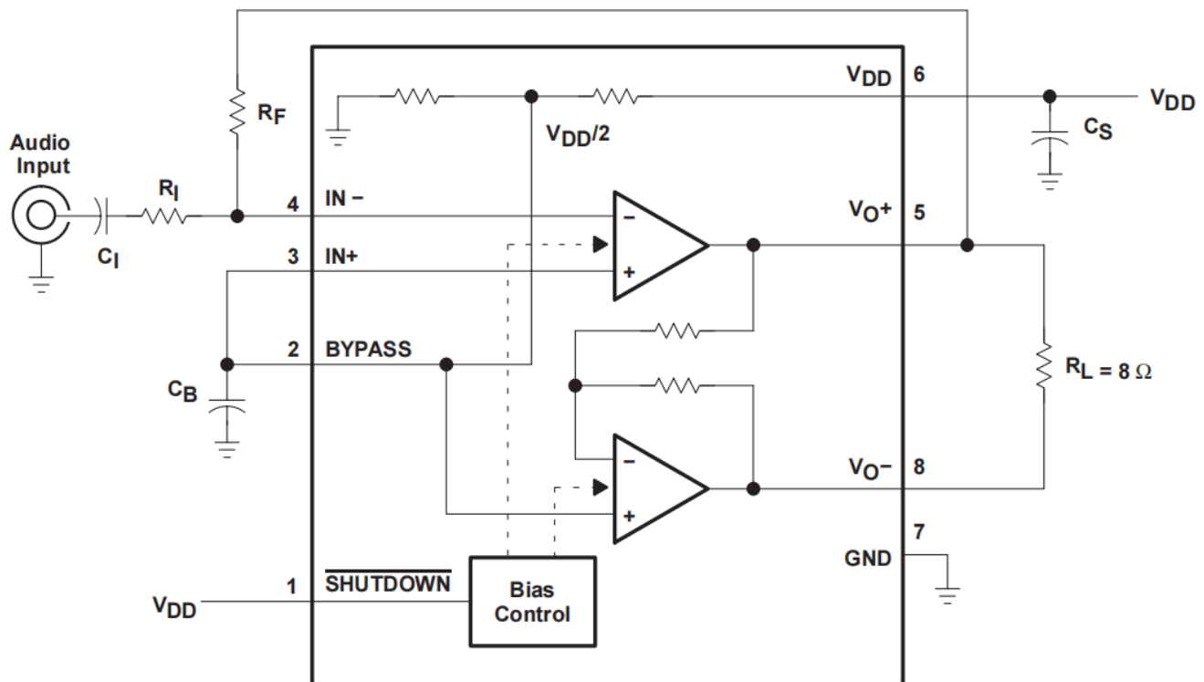
Figure 1. BTL Mode Test Circuit
