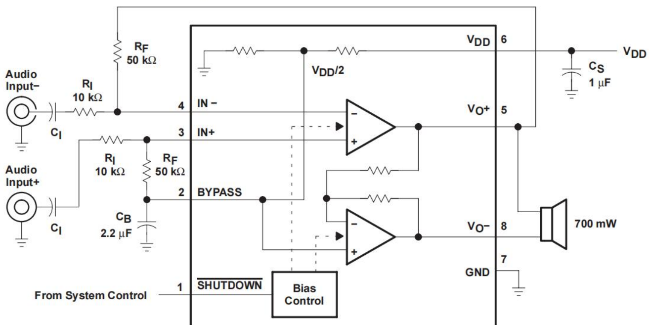
Figure 27. TPA751 Application Circuit With Differential Input
