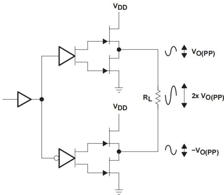
Figure 23. Bridge-Tied Load Configuration
