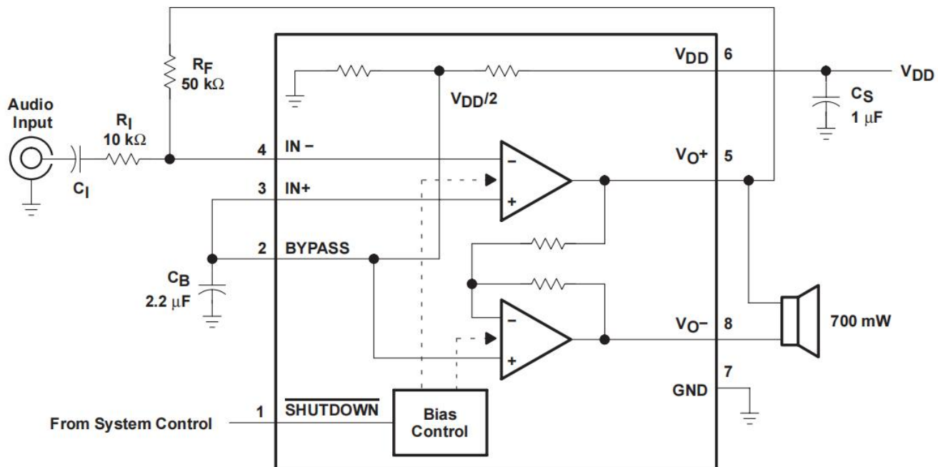
Figure 26. TPA751 Application Circuit
