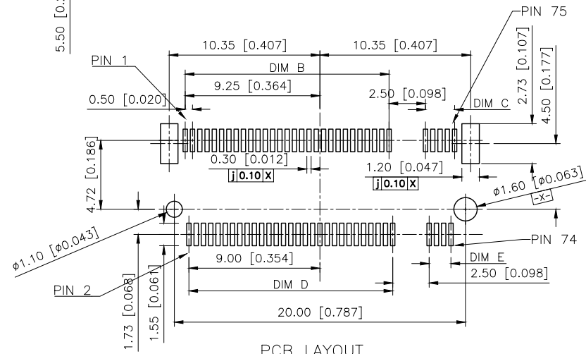
PCB LAYOUT
