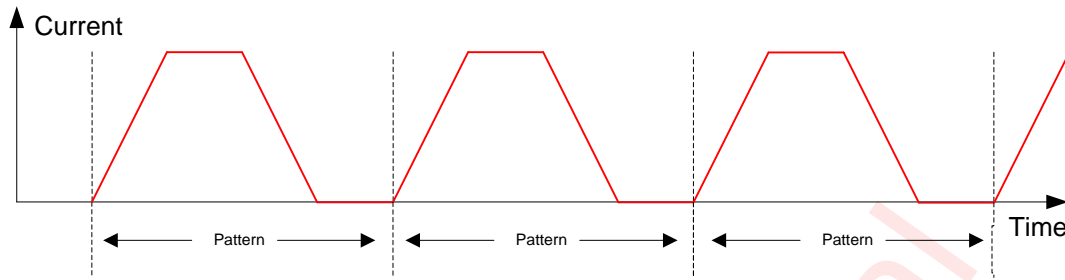
Figure 17. Example of single-pulse/single-color true-color pattern
