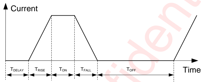
Figure 13. Basic single-pulse pattern parameter definition
