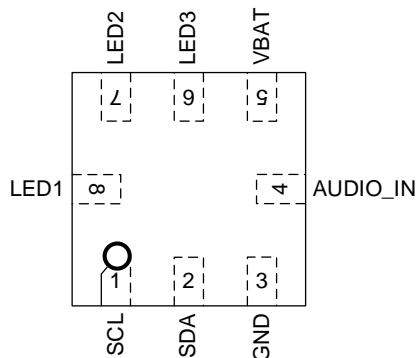
AW2028HFCR (Top View)
