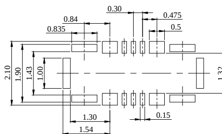
RECOMMENDED METAL DIMENSIONS (THICKNESS: 0.08 mm) DIMENSIONAL TOLERANCE: \pm 0.01
