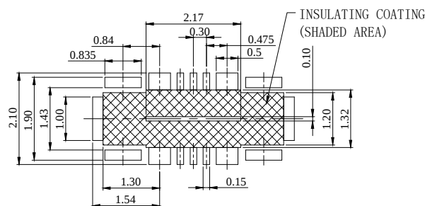
RECOMMENDED PCB LAYOUT DIMENSIONAL TOLERANCE: \pm 0.02
