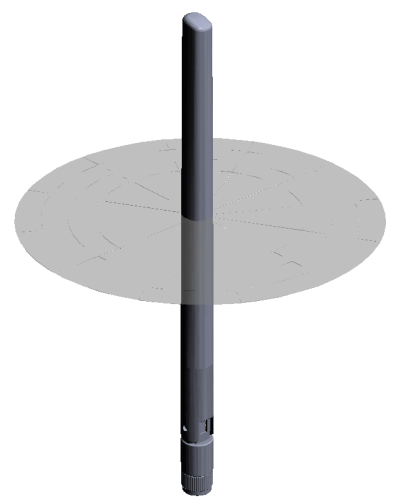
XY-Plane Gain
