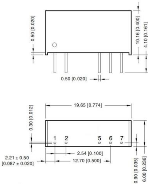
Figure 7: Overall dimensions 图7：外形尺寸
