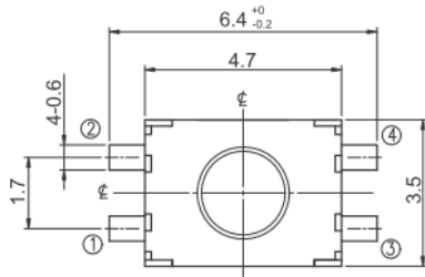
Figure 1 – 223AM..., Surface Mount Gull Wing
