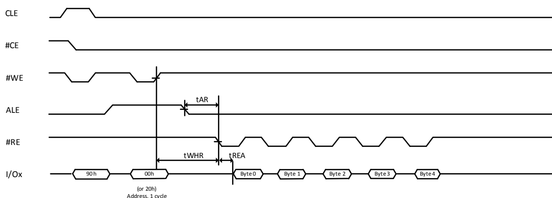
Figure 9-3 Read ID
