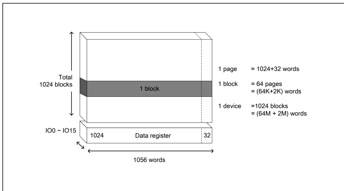
Figure 6-2 Array Organization
