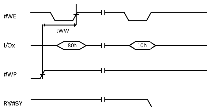
Figure 9-14 Program Enable
