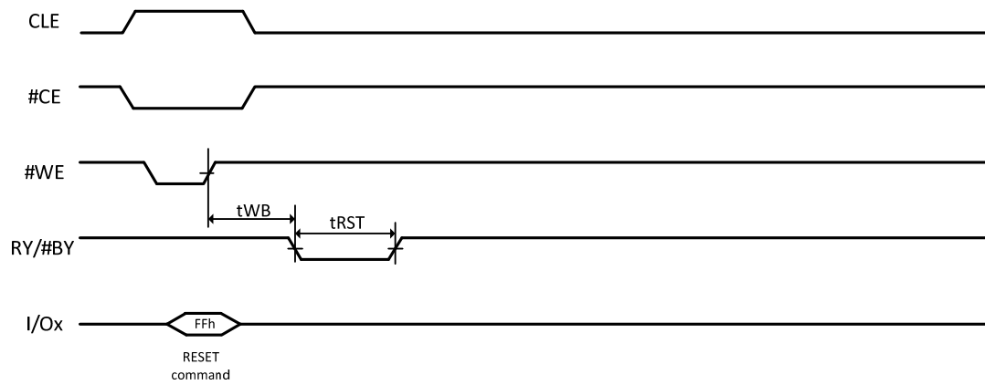
Figure 11-16 Reset
