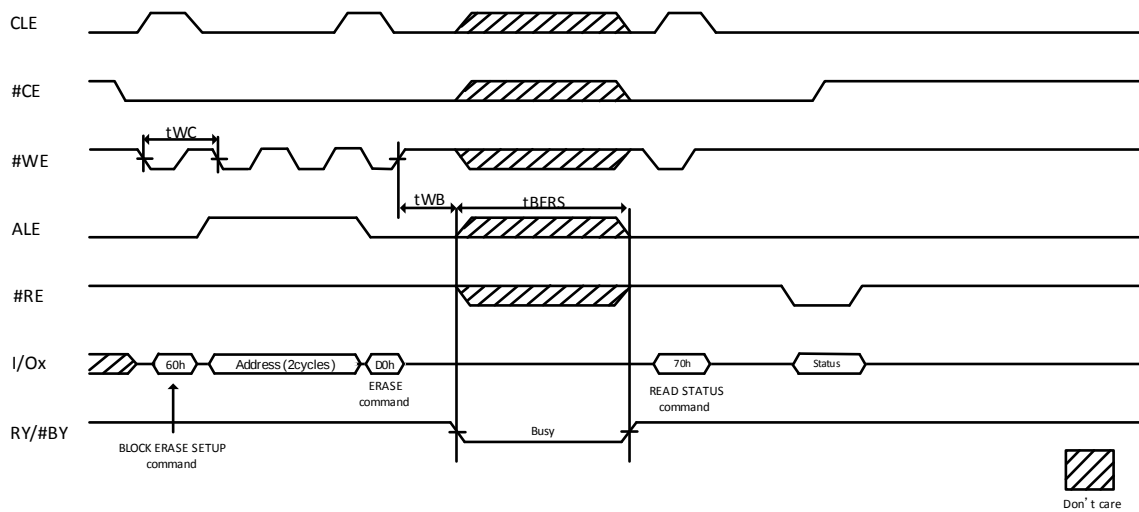
Figure 11-15 Block Erase
