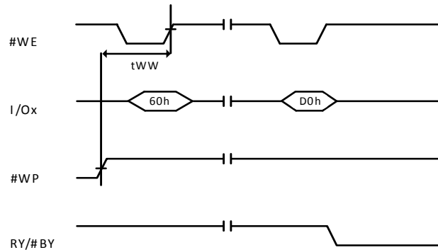
Figure 9-12 Erase Enable
