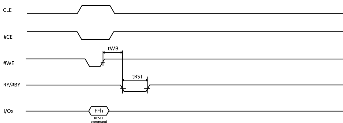
Figure 9-11 Reset Operation
