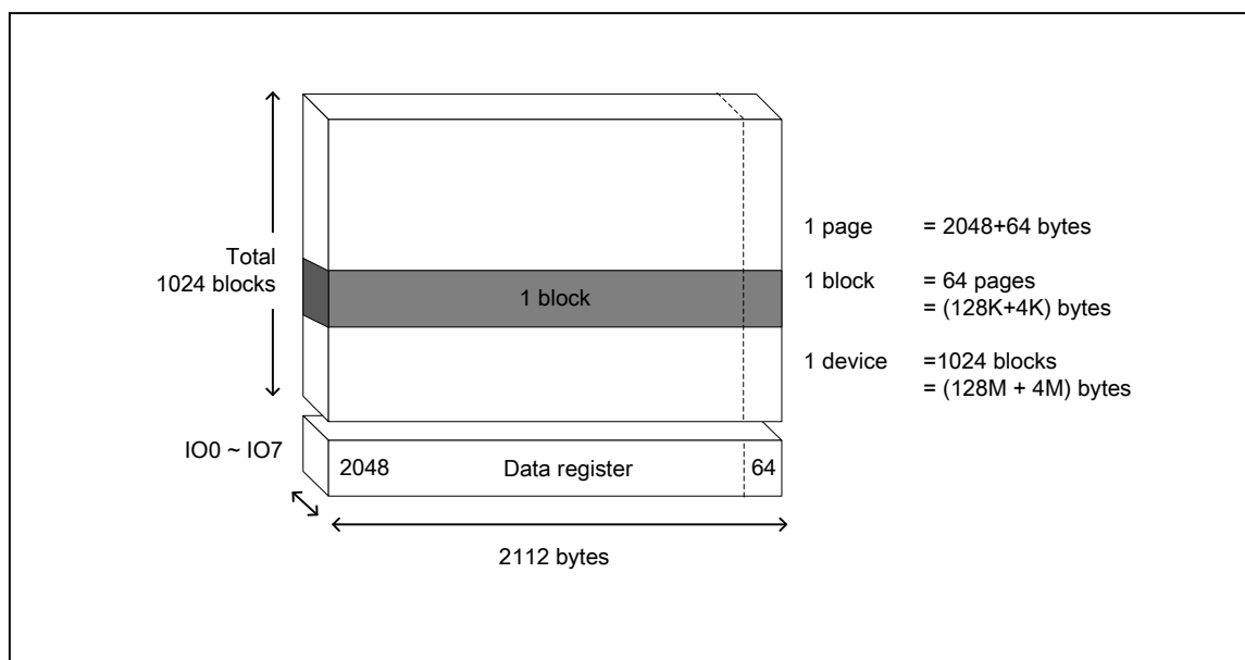
Figure 6-1 Array Organization
