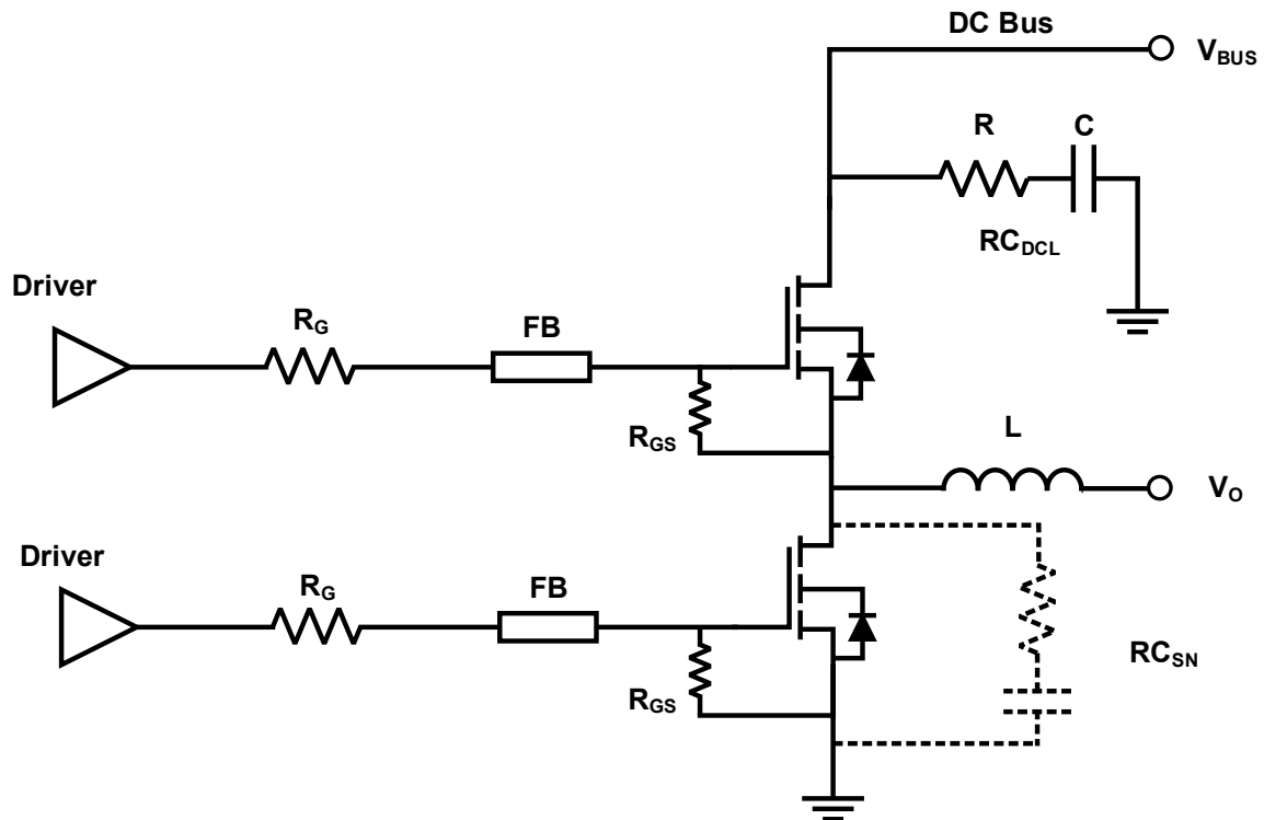
Figure 13. Simplified half-bridge schematic
