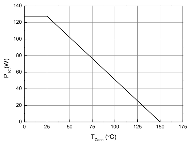
Figure 9. Power Dissipation
