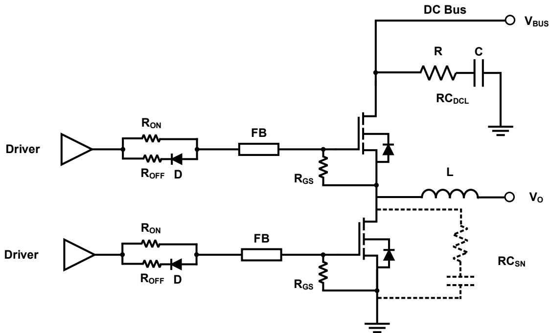
Figure 13. Simplified half-bridge schematic
