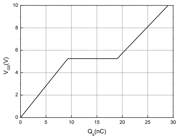
Figure 7. Typical Gate Charge ( I_{DS} = 22A , V_{DS} = 400V )
