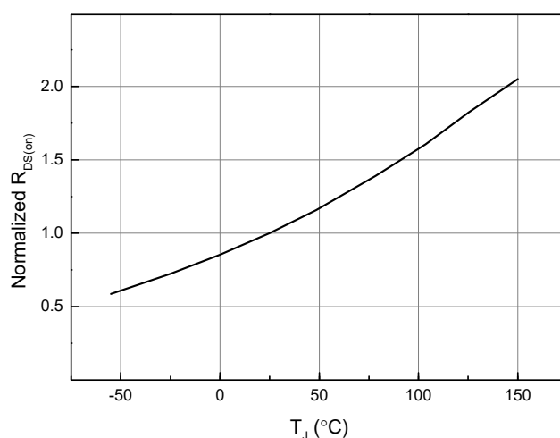
Figure 4. Normalized On-Resistance ( I_D = 22\text{A} , V_{GS} = 10\text{V} )
