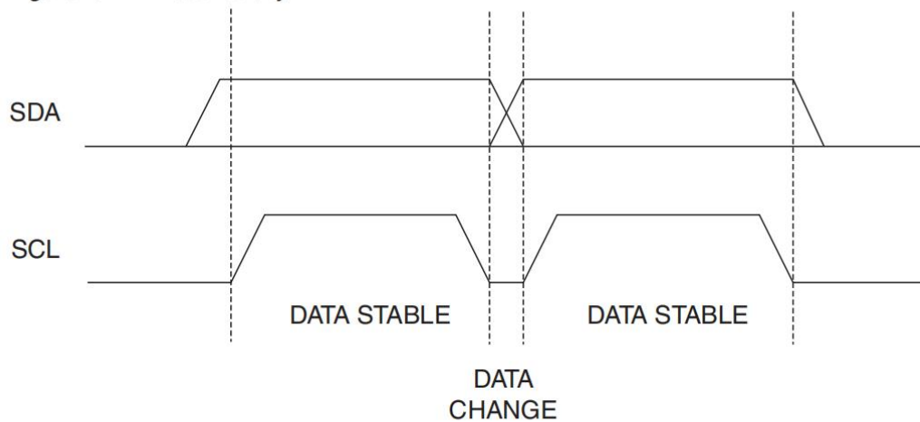
Figure 6. Data Validity
