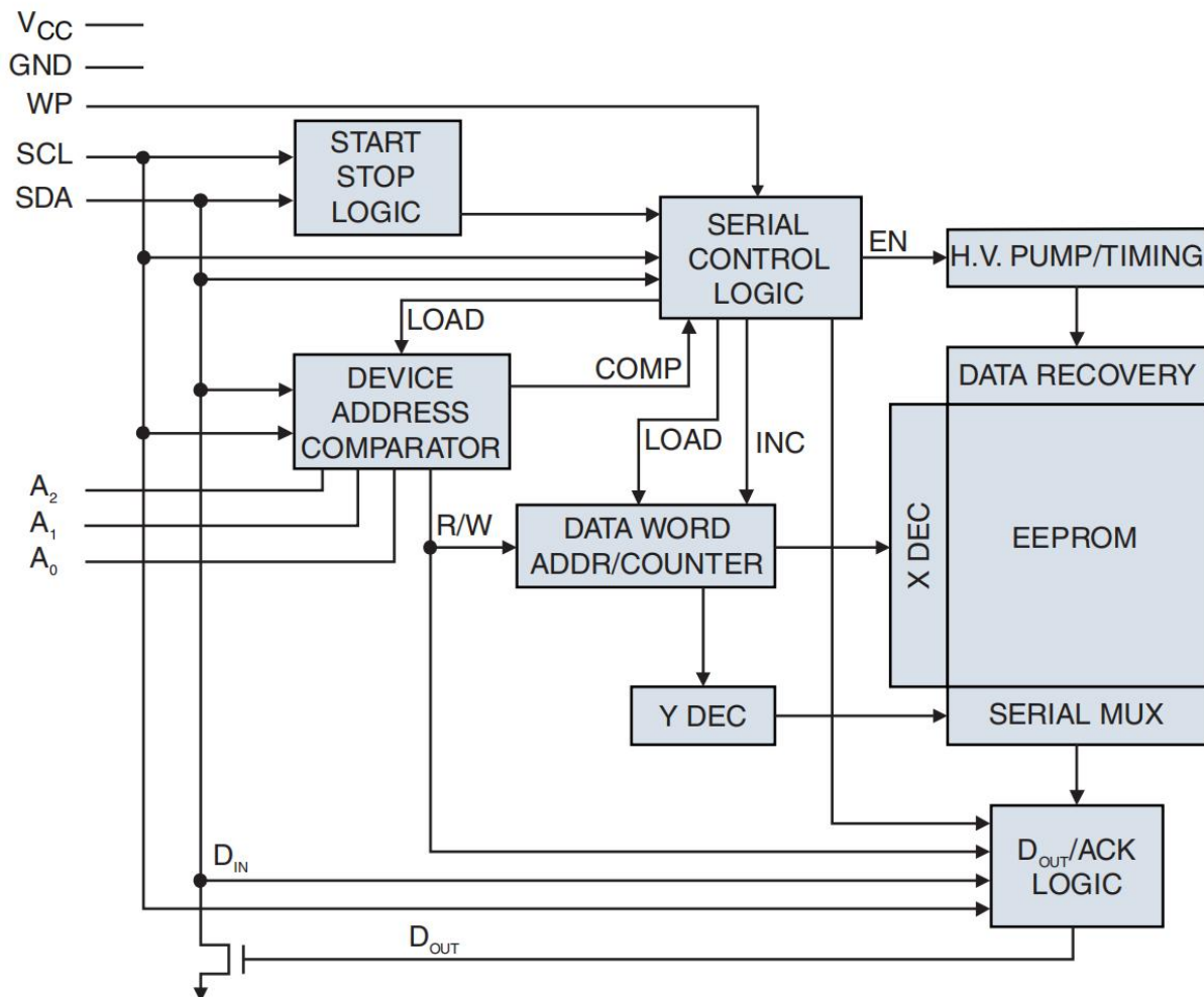
Figure 2. Block Diagram
