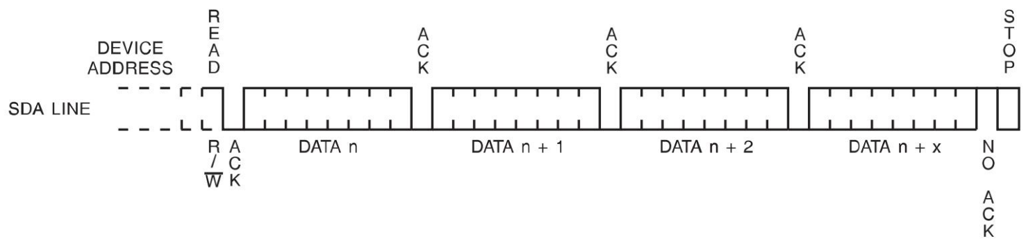
Figure 14. Sequential Read
