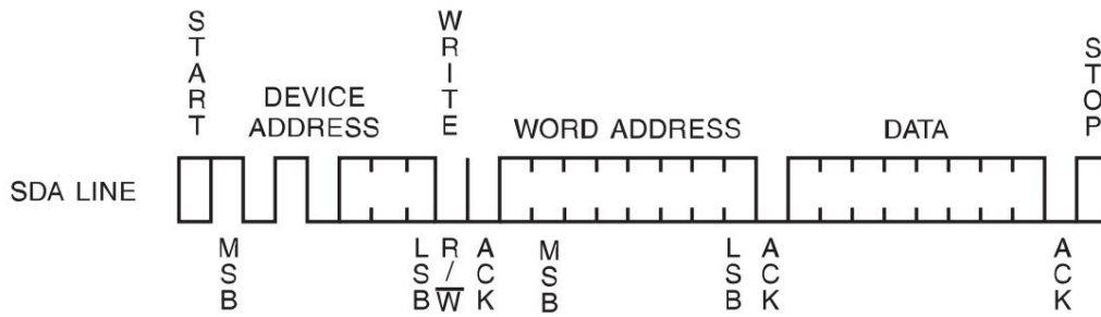
Figure 10. Byte Write
