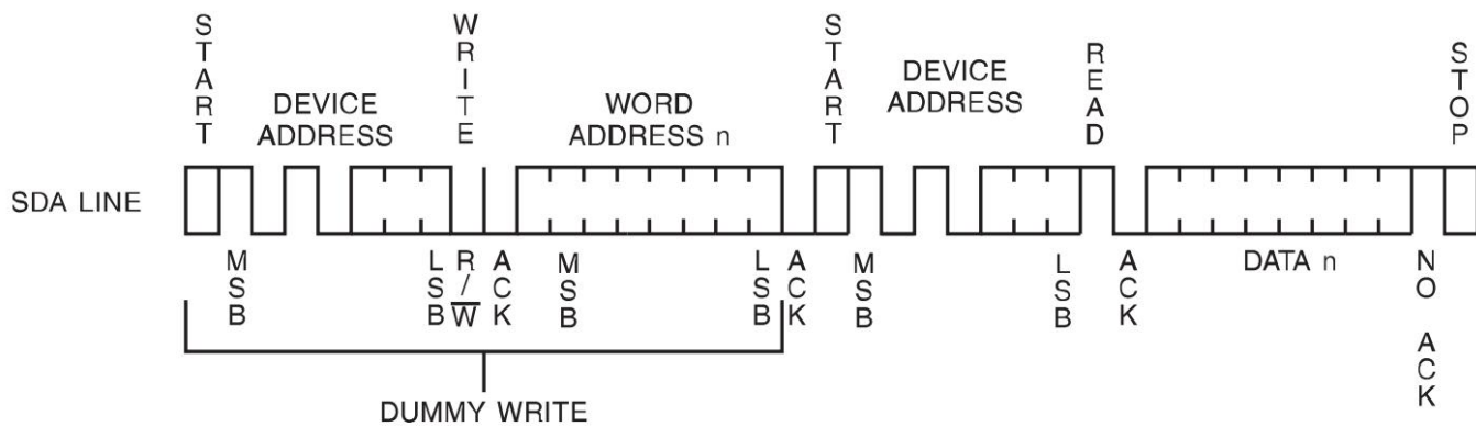
Figure 13. Random Read
