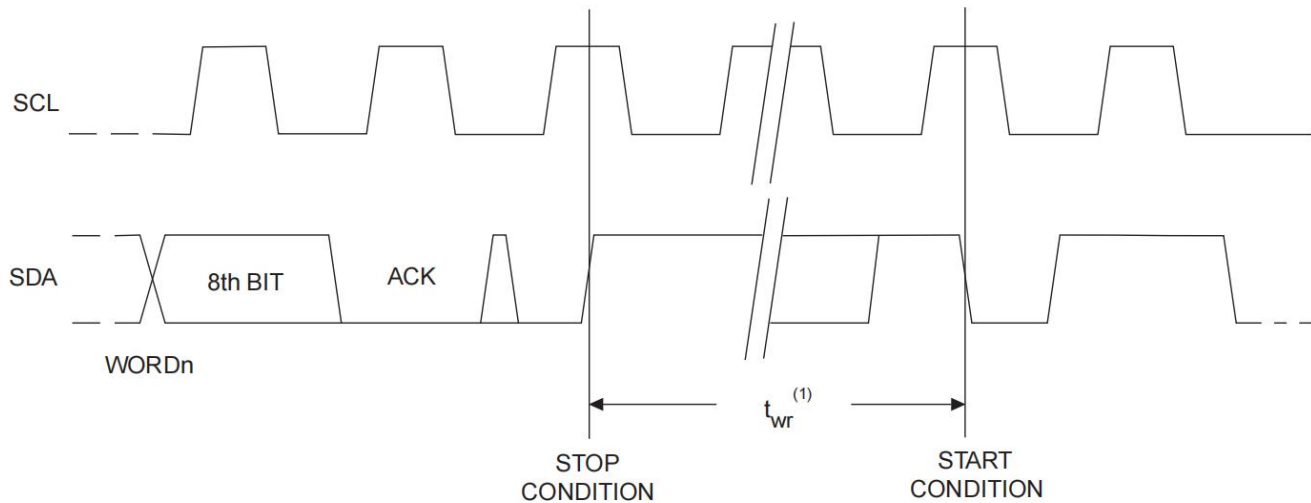
Figure 5. SCL: Serial Clock, SDA: Serial Data I/O
