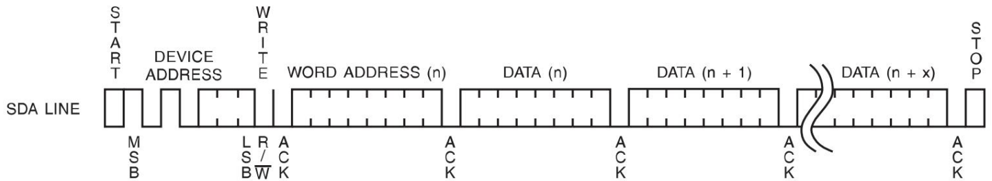
Figure 11. Page Write
