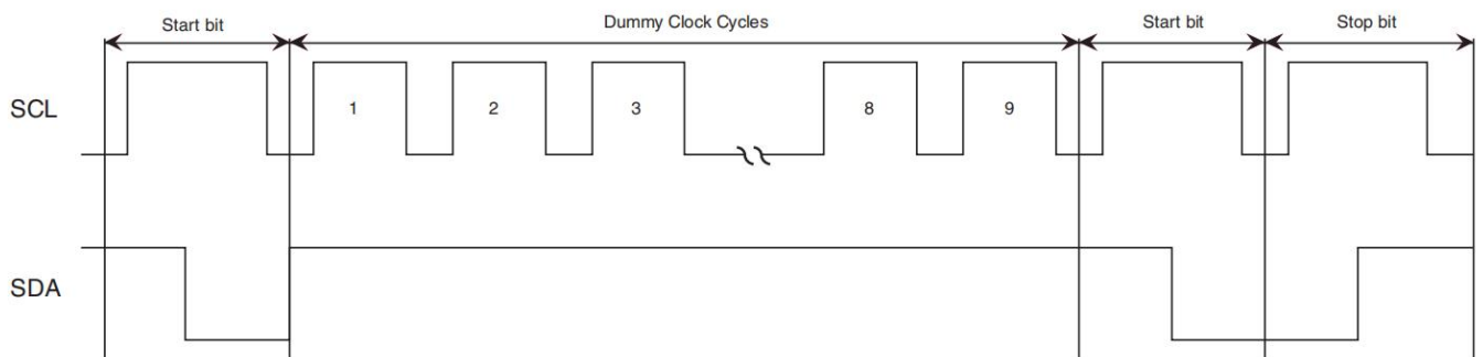
Figure 3. Software reset
