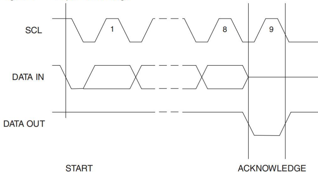
Figure 8. Output Acknowledge
