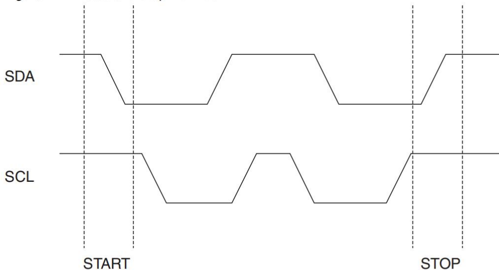
Figure 7. Start and Stop Definition
