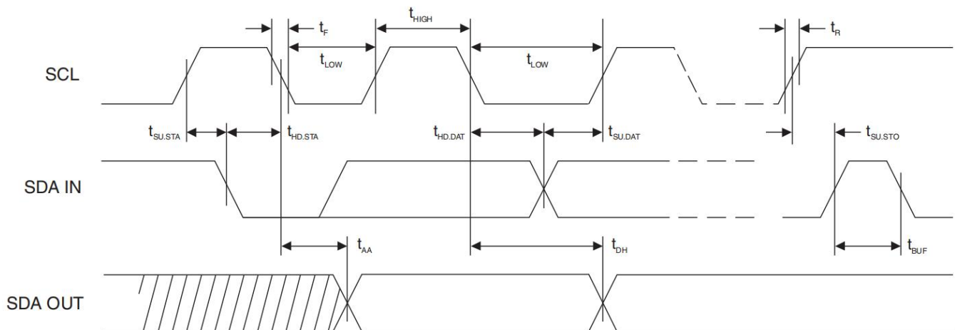
Figure 4. SCL: Serial Clock, SDA: Serial Data I/O®
