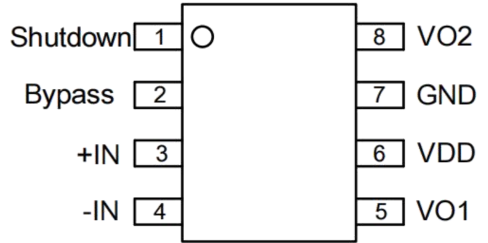
TPA301 Pin Diagram
