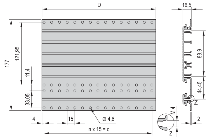
Extruded side panel 4 U, left
