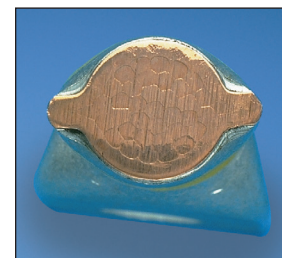
Crimped Lug Cross Section
