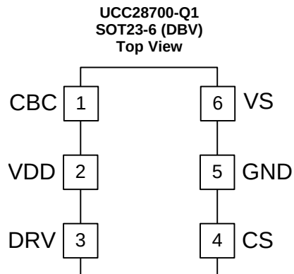
Pin Functions
