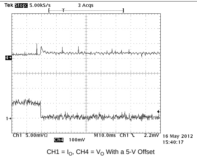
Figure 23. Load Transients: (0.6-A to 0.1-A Load Step)
