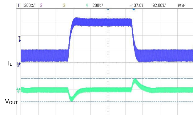
(16) Load Transient(VIN=50.0V,VOUT=12V,IOUT=0.1→0.6A)
