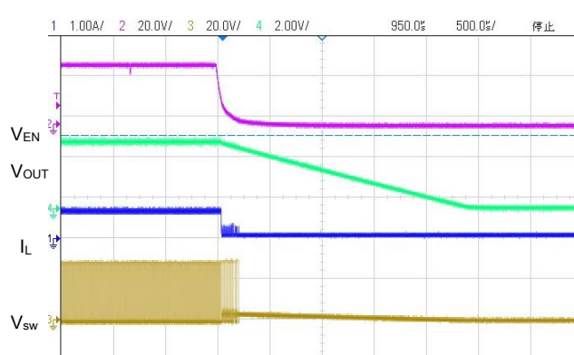
(18) Enable Shutdown(VIN=30.0V,VOUT=3.3V,IOUT=0.6A)
