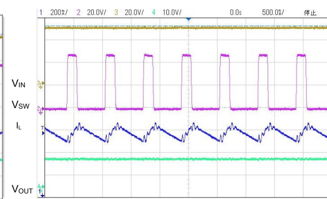
(24) Steady State ( V_{IN}=50.0V, V_{OUT}=12V, I_{OUT}=0.6A )
