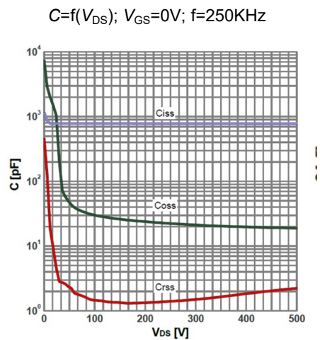
Figure 12:Typ. capacitances
