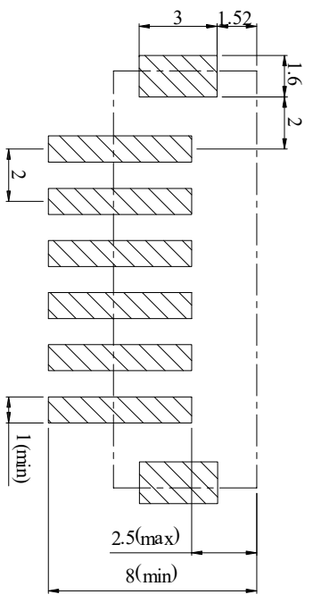
PCBLAYOUT
