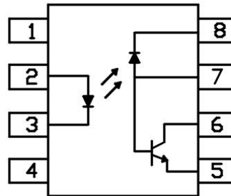
Pin Configuration
