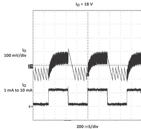
Figure 8-3. Load Transient Response
