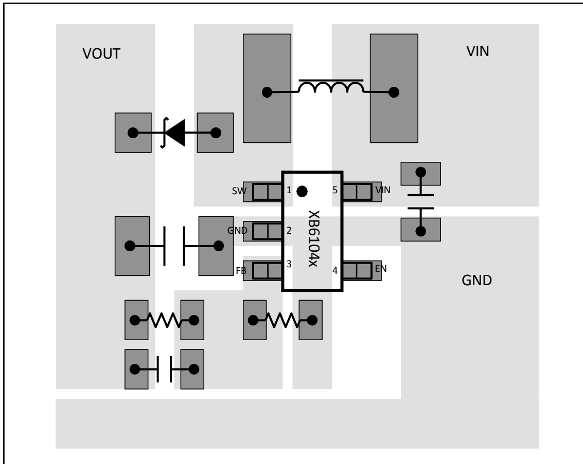
Figure 10-1.Layout
