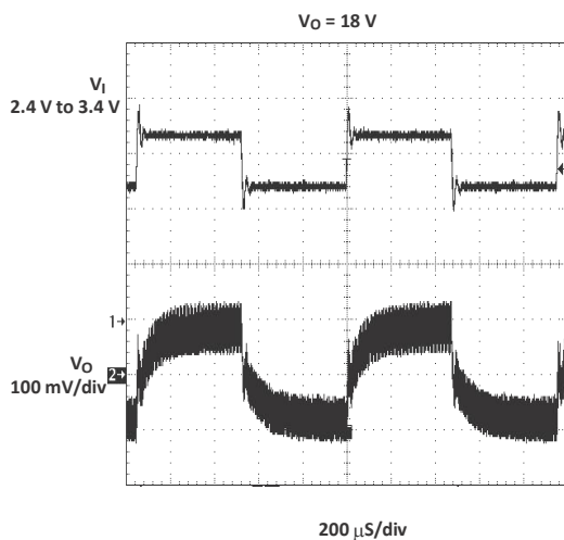
Figure 8-2. Line Transient Response
