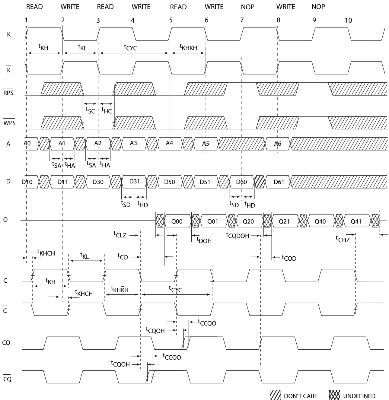
Figure 5. Read/Write/Deselect Sequence [31, 32, 33]
