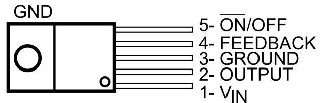
5-LEAD TO-263(U)
