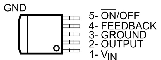
5-LEAD TO-263(U)
