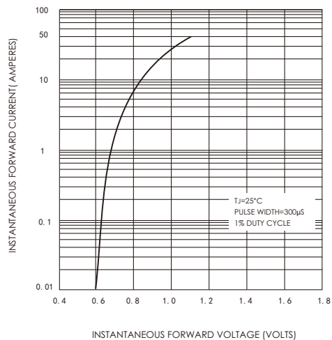
FIG.2-TYPICAL FORWARD CHARACTERISTICS
