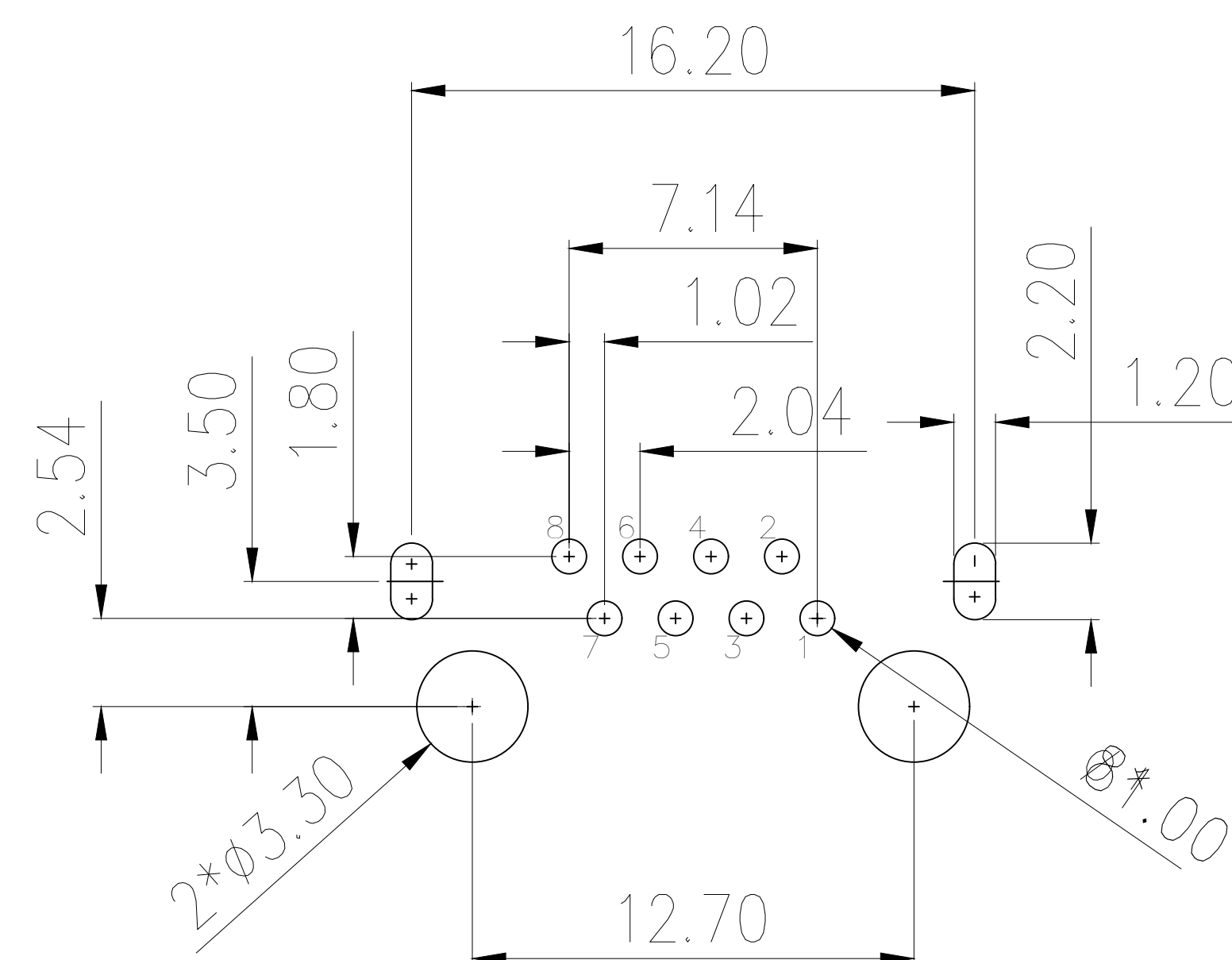
RECOMMENDER P. C. B. LAYOUT TOP VIEW (COMPONENT SIDE TOLERANCE \pm 0.05 )
