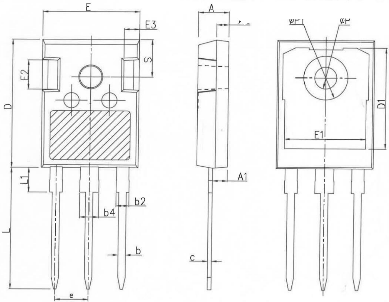
COMMON DIMENSIONS
