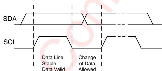
Figure 32 Data Validation Diagram
