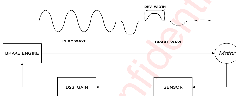
Figure 26 Brake loop
