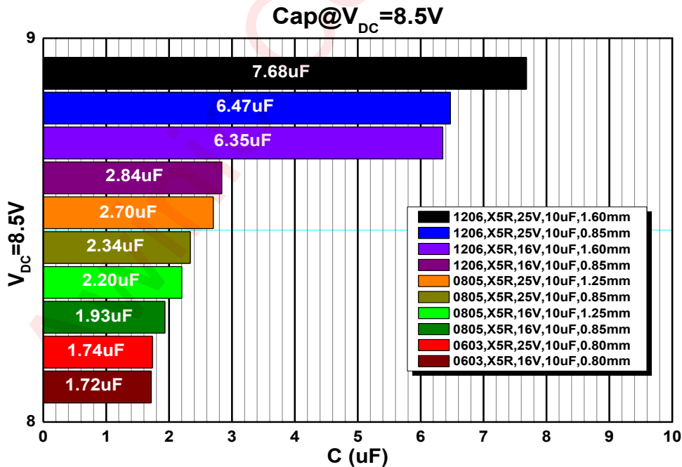
Figure 39 The space remaining value of different types of capacitors at V DC = 8.5 V
