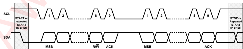
Figure 35 Data transmission on the I 2 C bus
