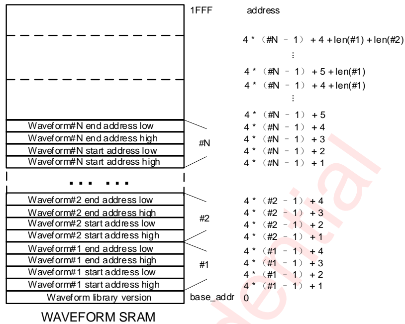
Figure 19 Waveform library data structure
