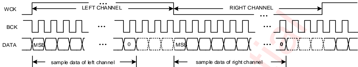
Figure 30 I 2 S Timing for Left-Justified Mode
