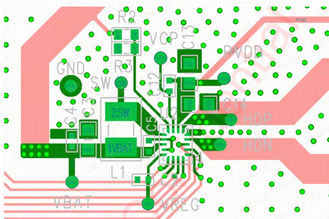
Figure 41 AW86937 Board Layout
