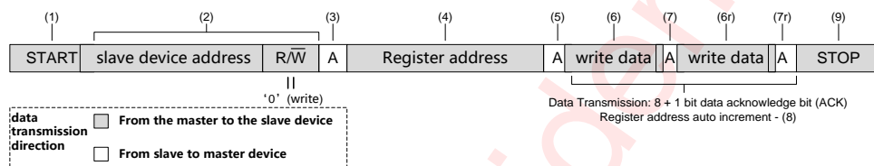
Figure 36 Writing process (data transmission direction remains the same)
