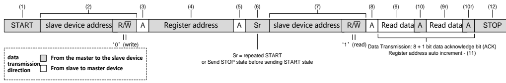
Figure 37 Reading process (data transmission direction remains the same)
