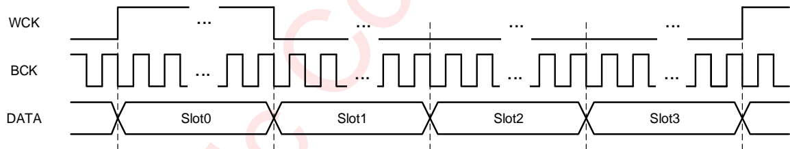
Figure 31 TDM Timing
