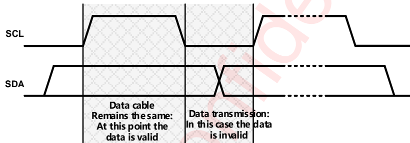
Figure 34 The data transfer rules on the I 2 C bus
