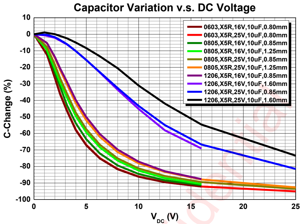
Figure 38 Different types of capacitive voltage stability
