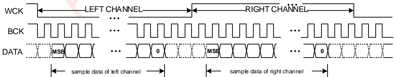
Figure 29 I 2 S Timing for Standard I 2 S Mode
