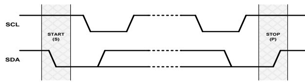
Figure 33 START and STOP state generation process
