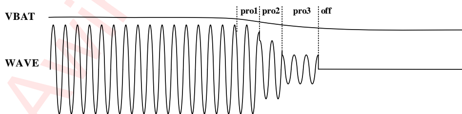
Figure 27 Battery protection process
