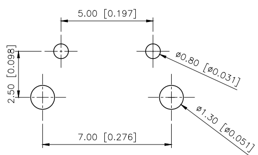
PCB.WELDING DRAWING
