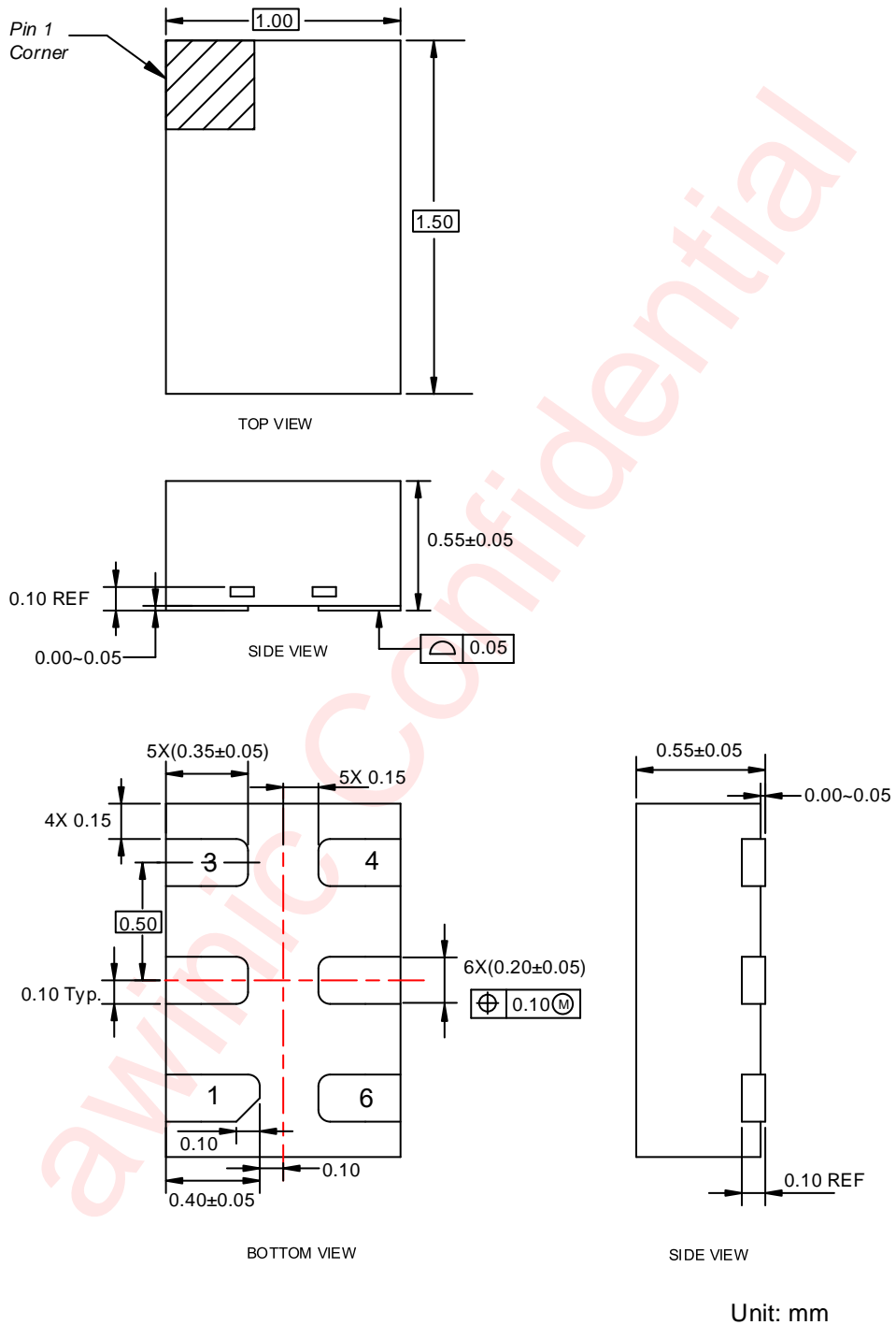
Figure 9 Package Outline
