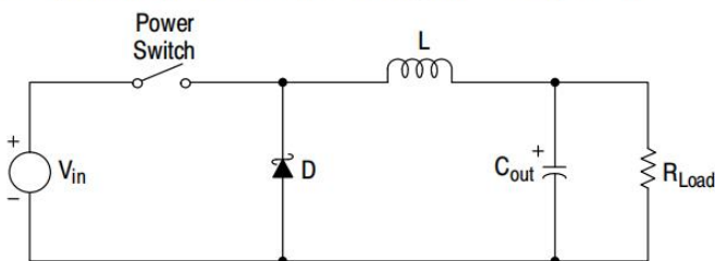
Figure 16. Basic Buck Converter
