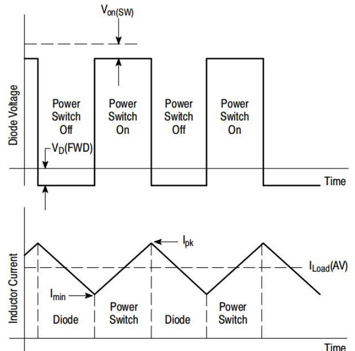
Figure 17. Buck Converter Idealized Waveforms
