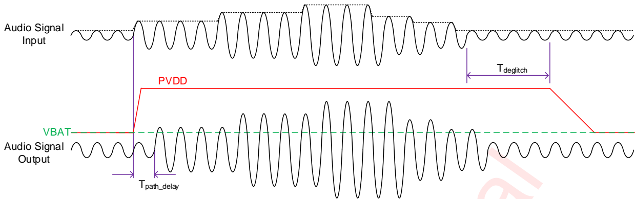
Figure 15 Boost Circuit Behavior in Smart Boost 1 Mode
