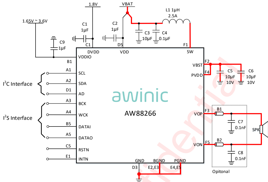
Figure 3 AW88266 Application Circuit
