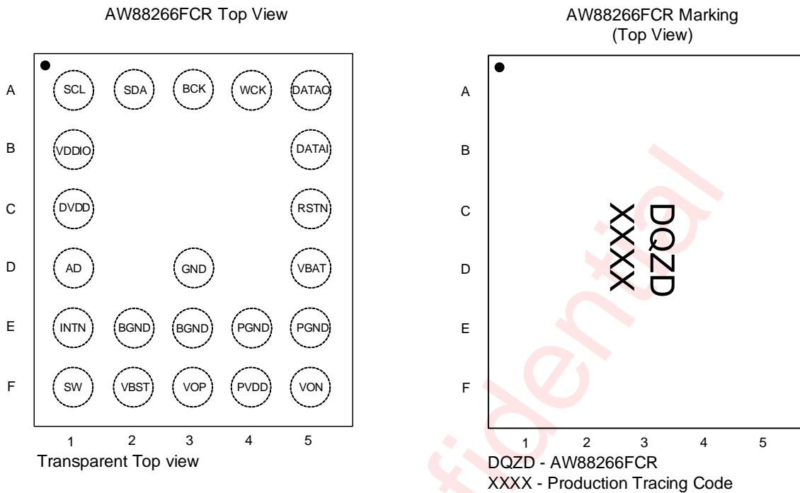
Figure 1 AW88266FCR pin diagram top view and device marking
