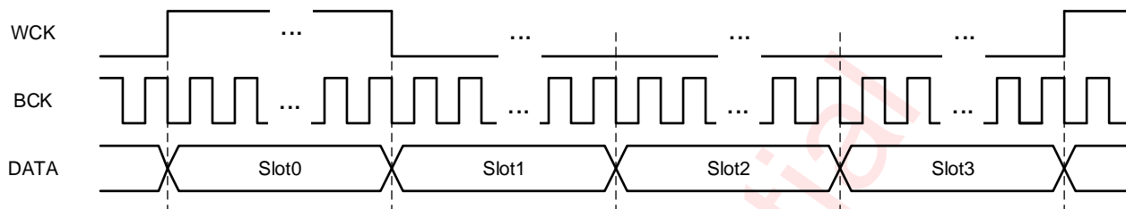
Figure 13 TDM Timing
