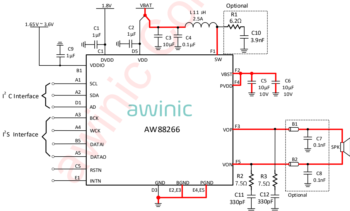
Figure 4 AW88266 Application Circuit (4Ω Load application)
