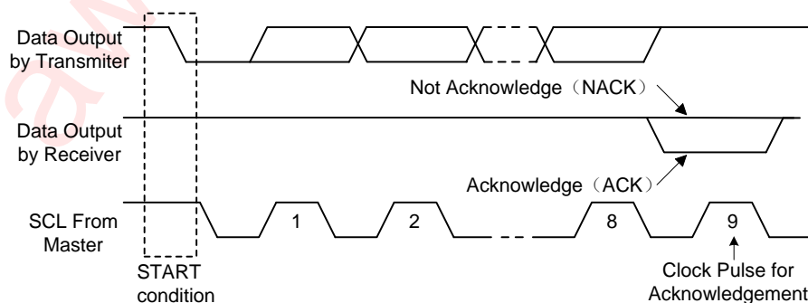
Figure 19 I 2 C ACK Timing
