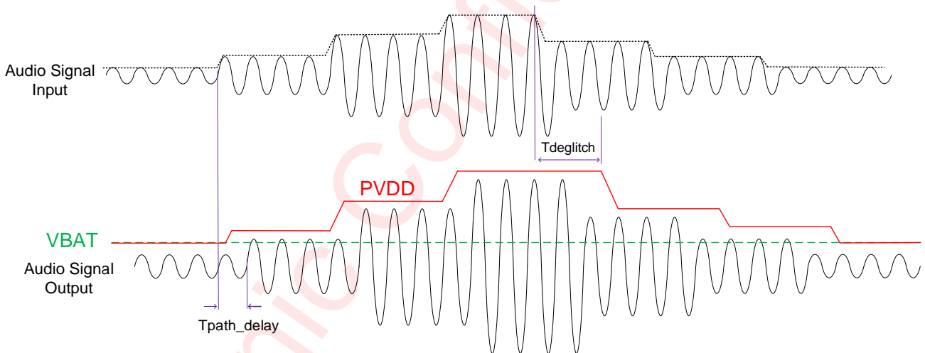
Figure 16 Boost Circuit Behavior in Smart Boost 2 Mode
