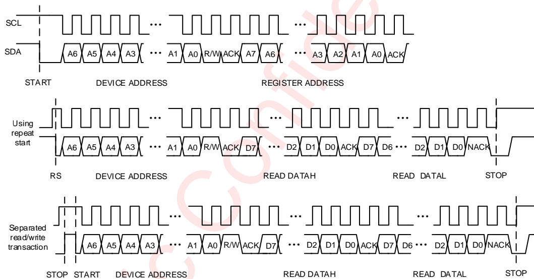
Figure 21 I 2 C Read Byte Cycle
