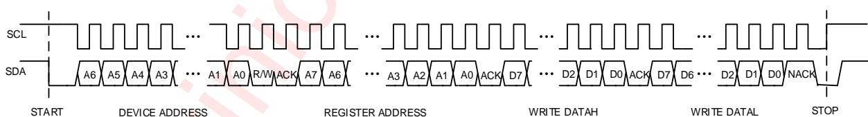
Figure 20 I 2 C Write Byte Cycle
