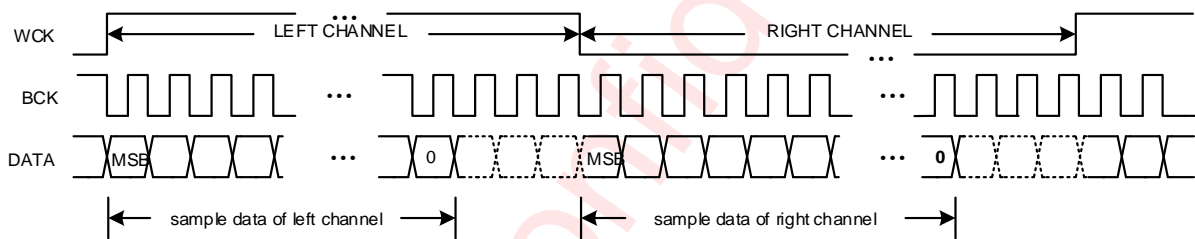
Figure 11 I 2 S Timing for Left-Justified Mode
