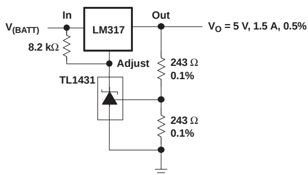
Figure 22. Precision 5-V, 1.5-A, 0.5% Regulator
