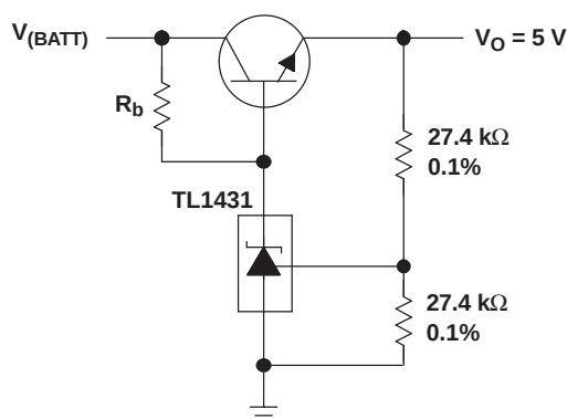
Figure 21. Crowbar
