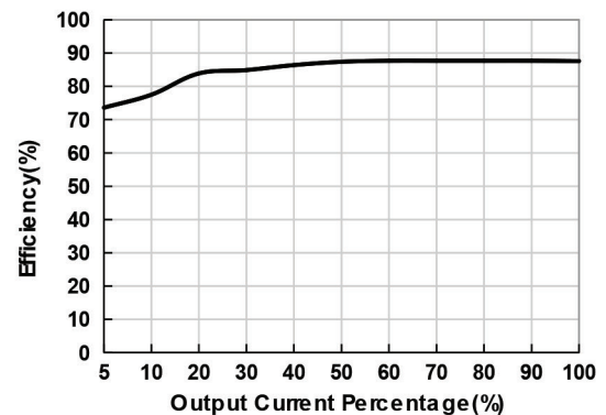
VXO7805-500-M Efficiency Curve Efficiency vs. Load Current ( V_{in} = 24\text{ V} )
