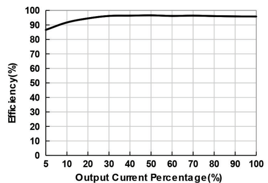
VXO78015-500-M Efficiency Curve Efficiency vs. Load Current ( V_{in} = 24\text{ V} )
