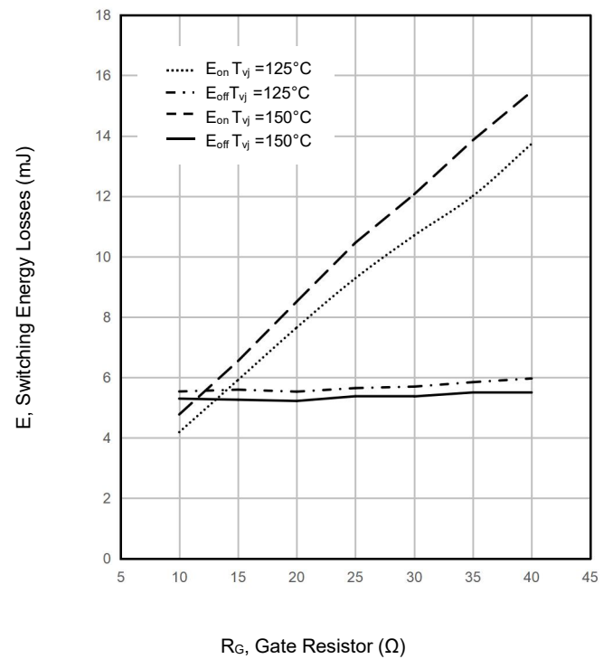
Figure 4. Switching Loss vs. R_G
