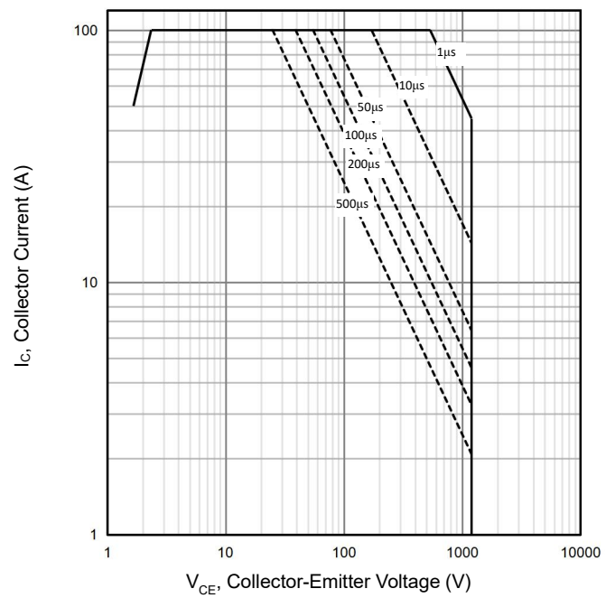
Figure 10.FBSOA IGBT
