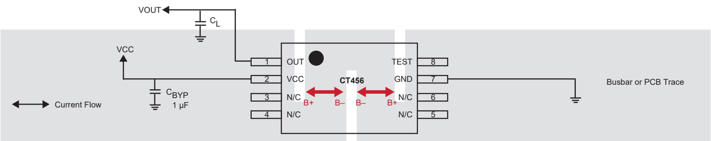
Figure 2: CT456 Application Diagram for Measuring Differential Magnetic Field for TSSOP-8
