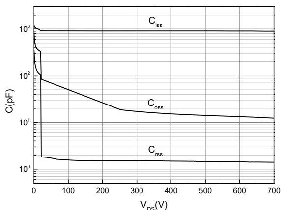
Figure 5. Typical Capacitance ( V_{GS} = 0V , f = 500kHz )
