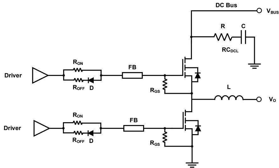
Figure 14. Simplified half-bridge schematic
