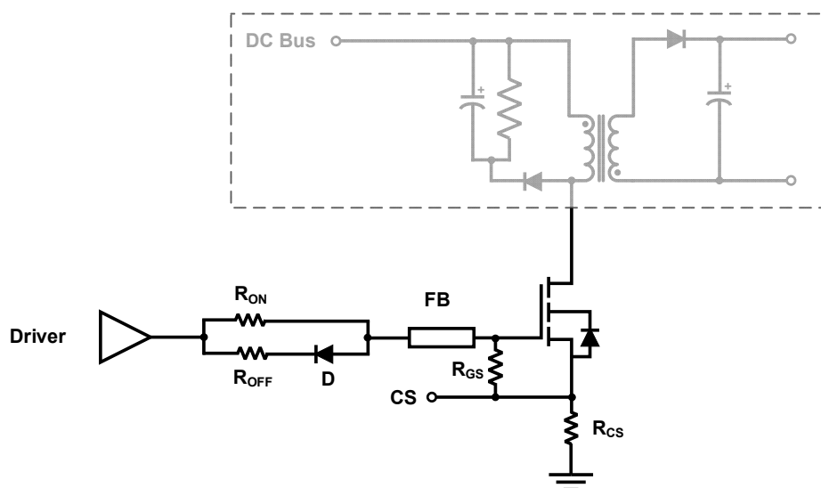
Figure 13. Simplified flyback schematic
