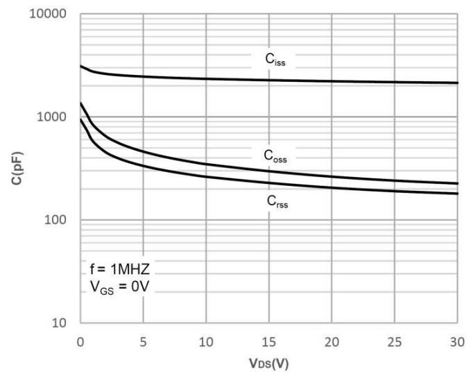
Capacitance Characteristics
