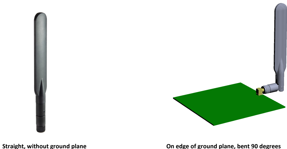
Figure 3. Antenna Test Orientation
