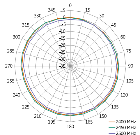
XY-Plane Gain
