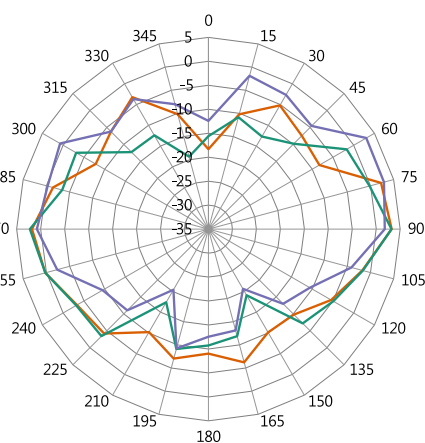
5550 MHz
