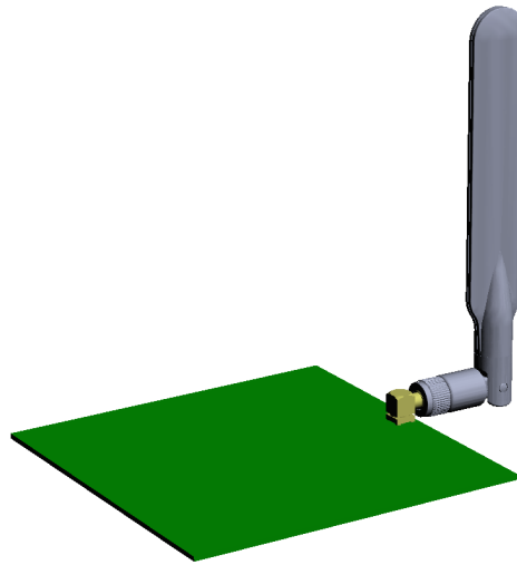
Figure 11. On edge of ground plane, Bent 90 Degrees
