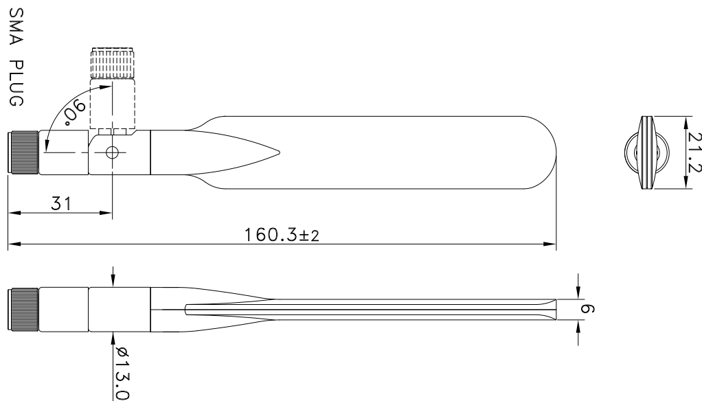
Figure 2. Antenna Dimensions
