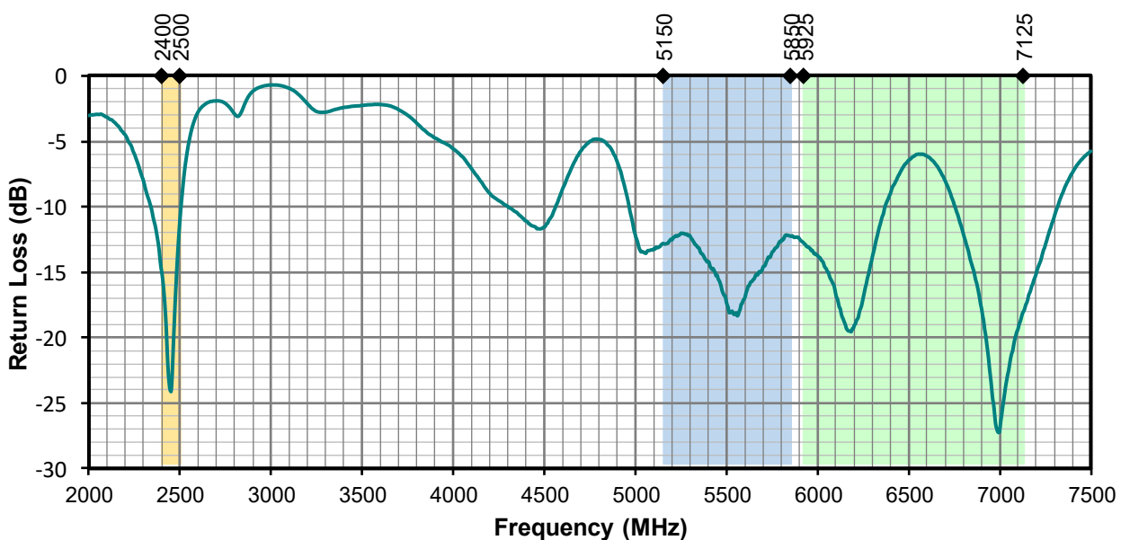
Figure 12. Antenna VSWR, Edge Bent 90 Degrees
