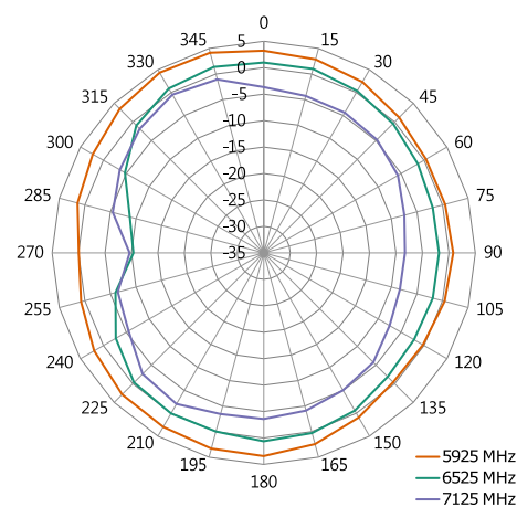
XY-Plane Gain
